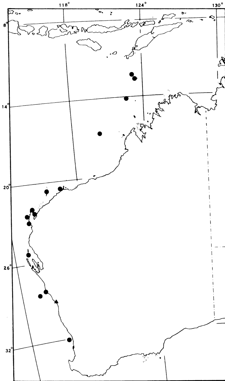
Figure 2 Map of Western Australia showing the distribution of living (●) and fossil (▲) Echinometra mathaei .
